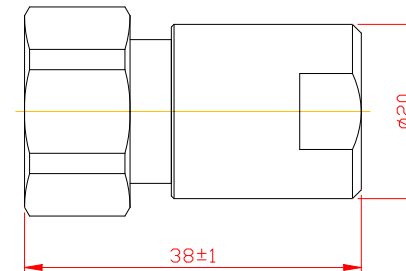
Outline Drawing
